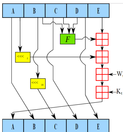
SHA-1 operation
