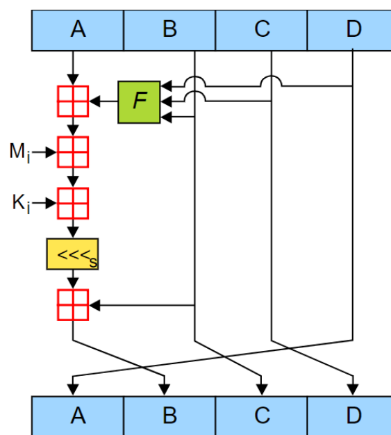
MD5 operation
